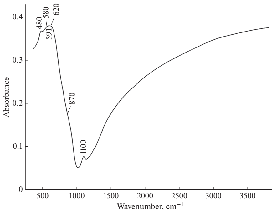
Fig. 2. Powder infrared absorption spectrum of nioboixiolite-(Mn 2+ ).
