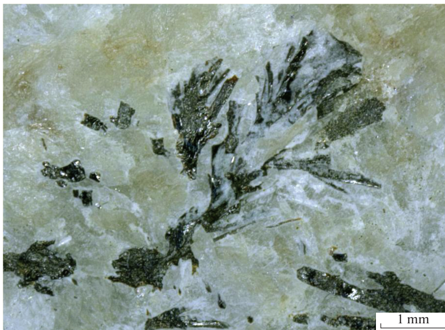
Fig. 1. Aggregates of nioboixiolite-(Mn 2+ ) in albite.
