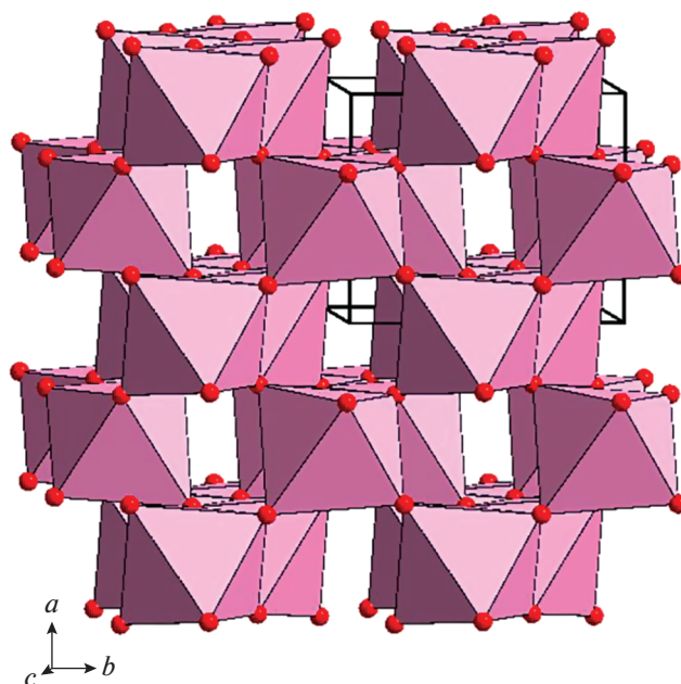
Fig. 3. The crystal structure of nioboixiolite-( \text{Mn}^{2+} ). The unit cell is outlined.
