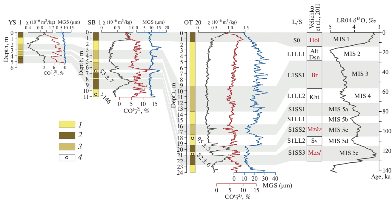
Fig. 3. Sublatitudinal cross-section of loess-paleosol sequences of the Upper Pleistocene and Holocene. OSL dates of SB-1 are from Mazneva et al. (2021). Other data is original. Subdivisions of scheme of Velichko et al. (2011): Hol – Holocene soil, Alt – Altynovo loess, Dsn – Desna loess, Br – Bryansk paleosol, Kht – Khotylevo loess, Mzkr – Krutitsa paleosol (upper phase of Mezin pedocomplex), Sv – Sevsk loess, Mzsl – Salyn paleosol (lower phase of Mezin pedocomplex). L/S – modern modification of Velichko scheme (Mazneva et al., 2021; Chen et al., 2022). Figure captions: 1 – loess, 2 – well-developed soil, 3 – weakly developed soil, 4 – OSL dates (ka).
