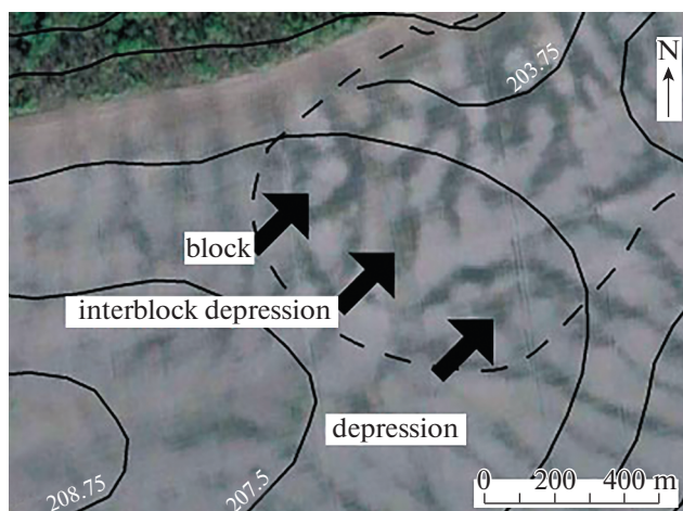
Fig. 2. Blocks and interblock depressions in the watershed area (for the slope of southern exposure); very high resolution satellite image courtesy of DigitalGlobe Foundation.
