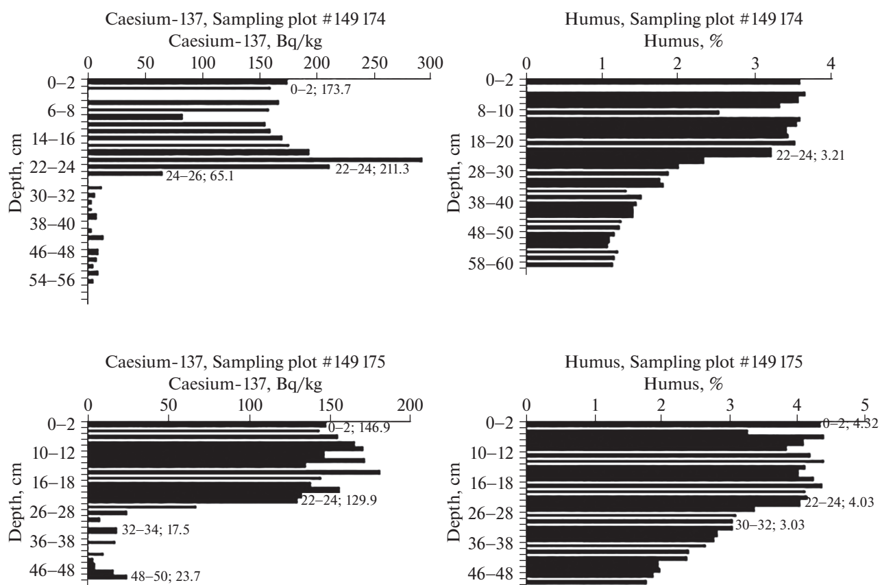
Fig. 5. In depth distribution of caesium-137 and humus; Sampling plot #149 174 is accepted when establishing background value (is located in block elevation); Sampling plot #149 175 is not accepted (is located in plowing furrow).
