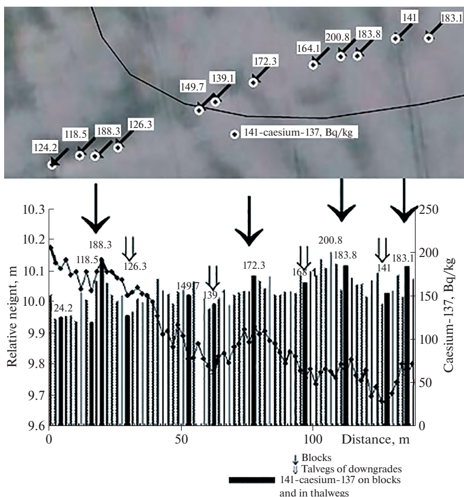
Fig. 4. A levelling profile combined with the radioactivity plot of caesium-137 (transect #91 224); and the transect location in a satellite image; very high resolution satellite image courtesy of DigitalGlobe Foundation.
