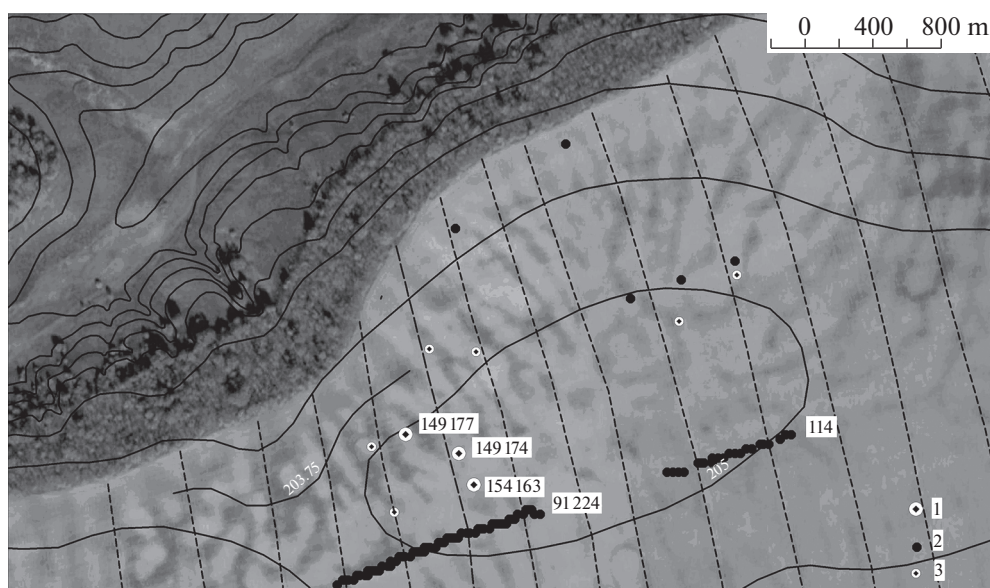
Fig. 3. Soil sampling transects at the watershed.
