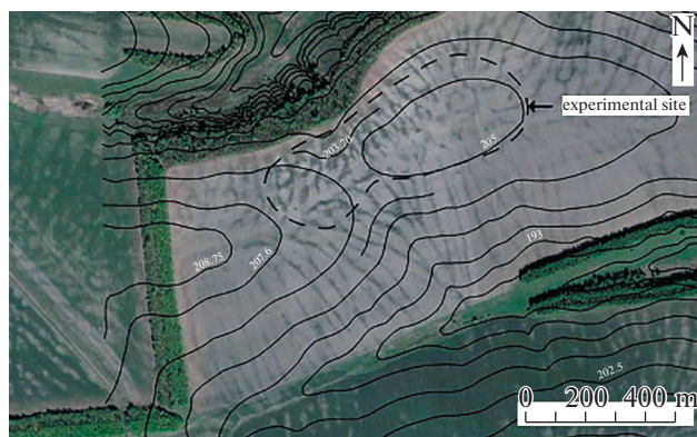
Fig. 1. An experimental area in the Sukhaya Orlitsa River basin; very high resolution satellite image courtesy of DigitalGlobe Foundation.
