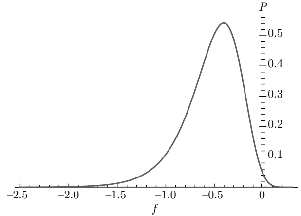
Critical free energy distribution function P(f) of the disordered Ising ferromagnet in dimension D = 3
