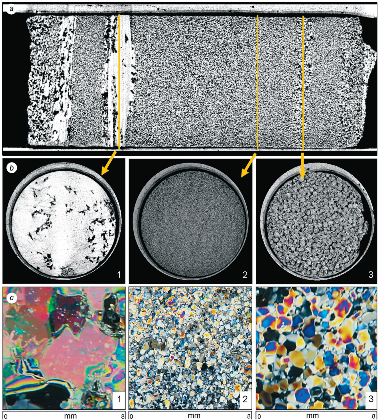
Fig. 5. The inner structure of the ice core: a – stereological visualization of the section 43; yellow lines with arrows indicate the cross sections; b – cross-sections of the core: 1 – ice (white color); 2 – fine-grain firn (dark gray color); 3 – coarse-grain firn (gray color); c – thin sections from the same horizons with crystals of: 1 – ice; 2 – fine-grain firn; 3 – coarse-grain firn
